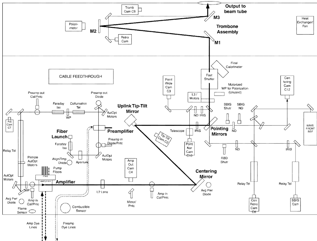
FIG. 8.—Schematic view of the 1.2 \times 1.8 m laser table and the trombone assembly mounted on the elevation ring of the telescope. The dark solid line shows the optical path from the laser amplifier cell off of the centering mirror, UTT mirror, and pointing mirror, through a three-mirror trombone assembly to the output up the beam tube. A portion of the light is split off at or near the pointing mirror to several diagnostics cameras. The light path prior to the amplifier begins at the fiber launch (a single-mode fiber from the dye master oscillator on the dome floor) and passes through the preamplifier and various formatting optics.
