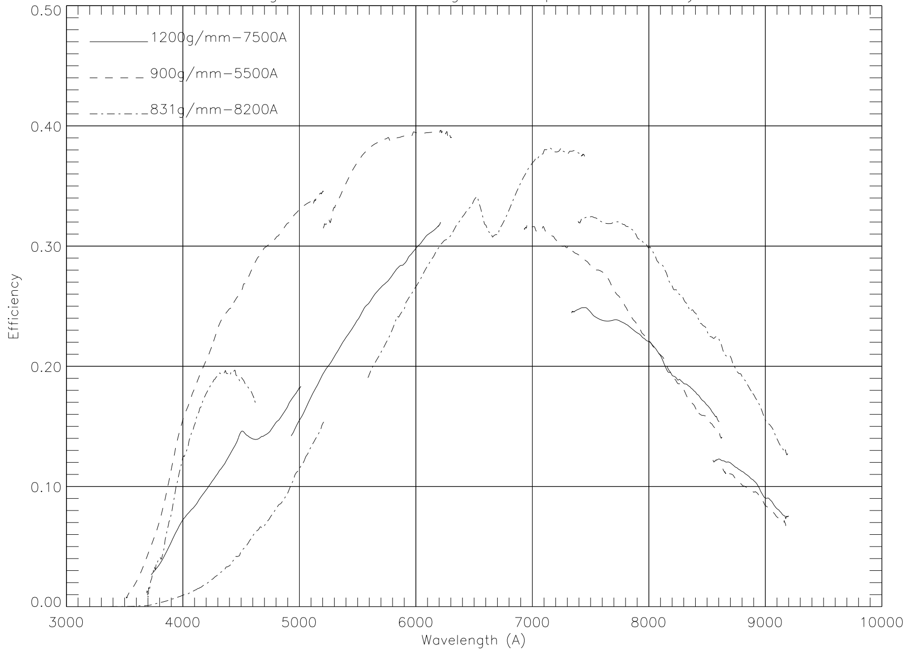
High-resolution Gratings LRIS Spectral Efficiency
