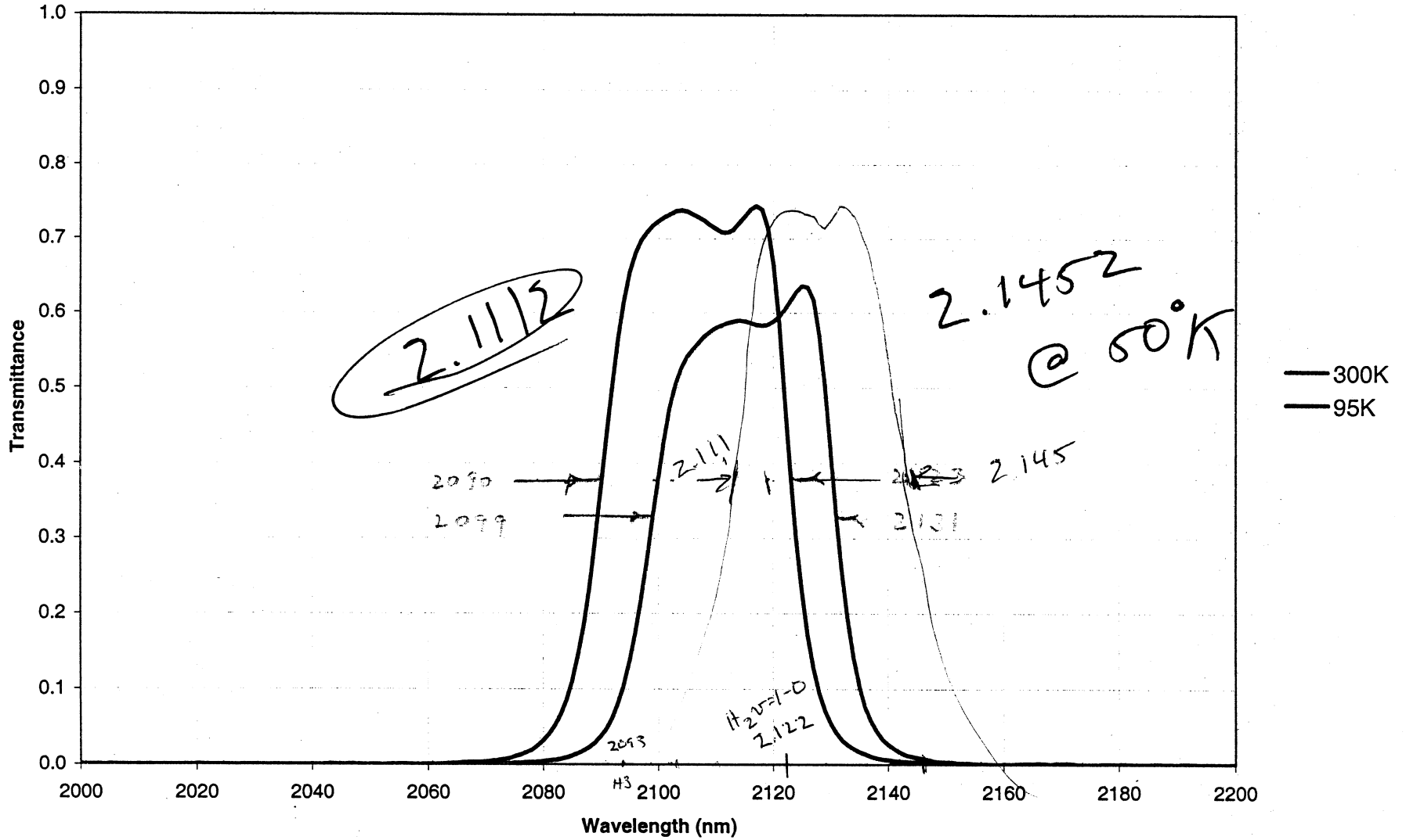
Representative temperature calibration spectra of batch 220600
