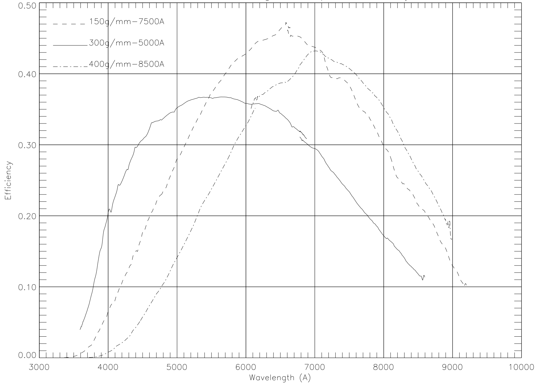
Low-resolution Gratings LRIS Spectral Efficiency
