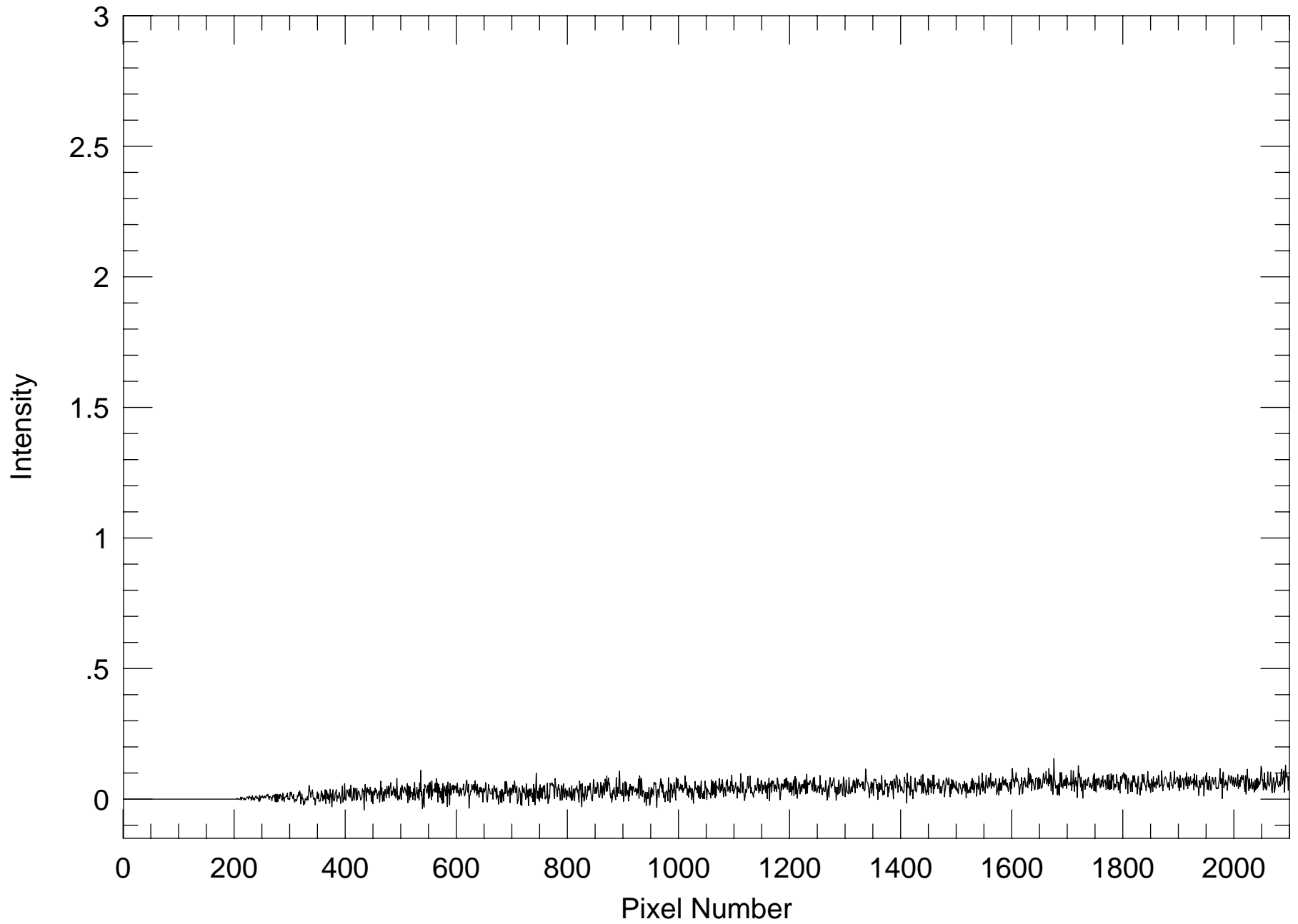
Xe, order 15, blue
