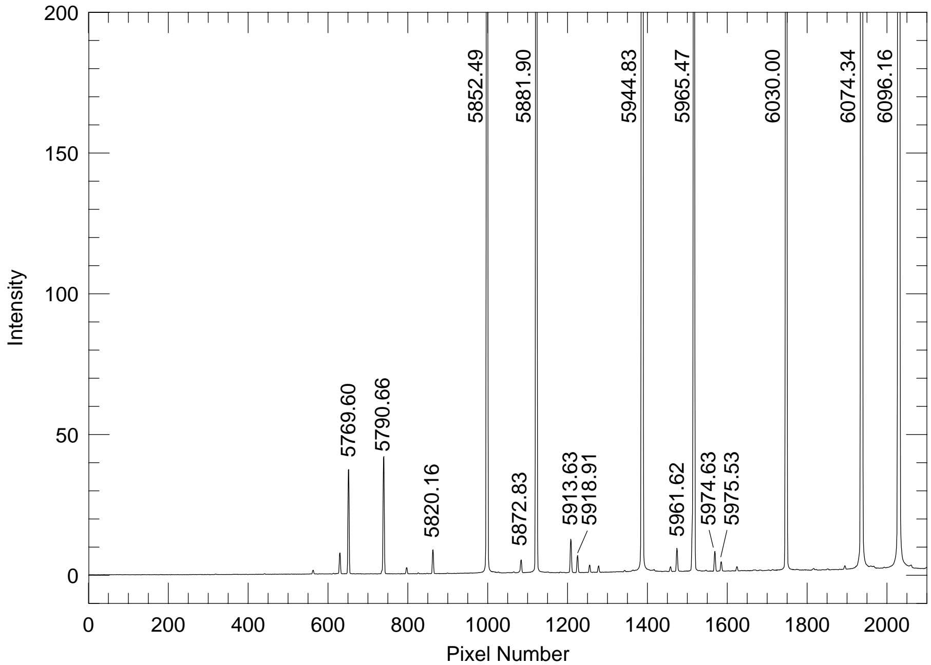
HgNe, order 10, blue
