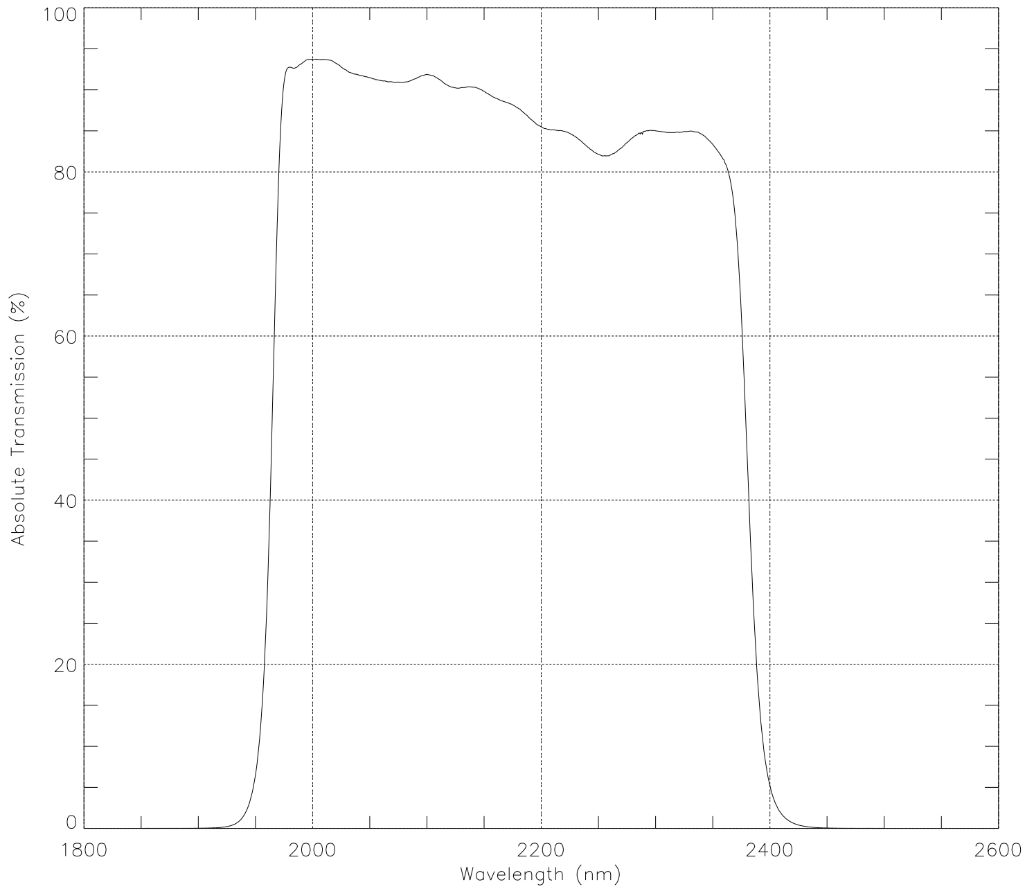
OSIRIS Filters – IMAG Kbb
